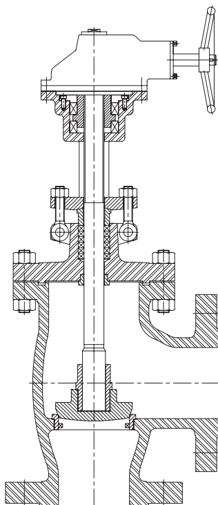
ANGLE STOP CHECK VALVE
