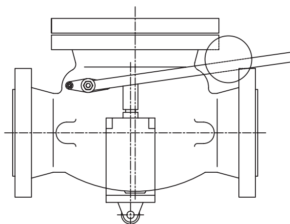
SWING CHECK VALVE WITH SLAM RETARDER
