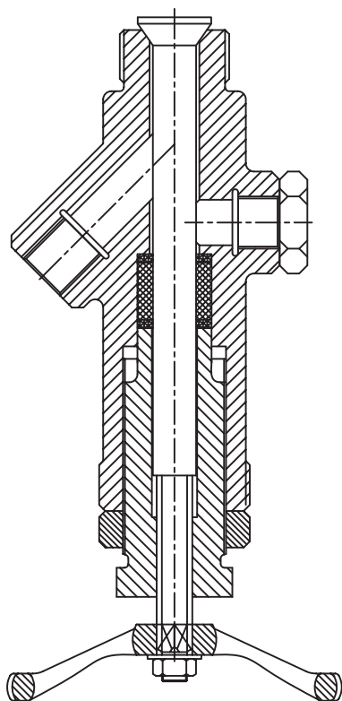
STEAM INJECTION VALVE
