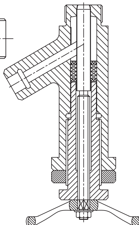
SAMPLING VALVE
