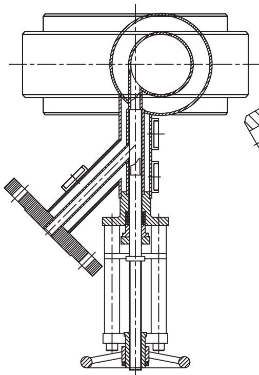
JACKETED SAMPLING VALVE WITH JACKETED TEE
