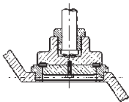
SOFT SEATED PLUG
