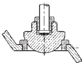
PARABOLIC PLUG
