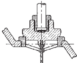
GUIDED PLUG SIZES > 6"
